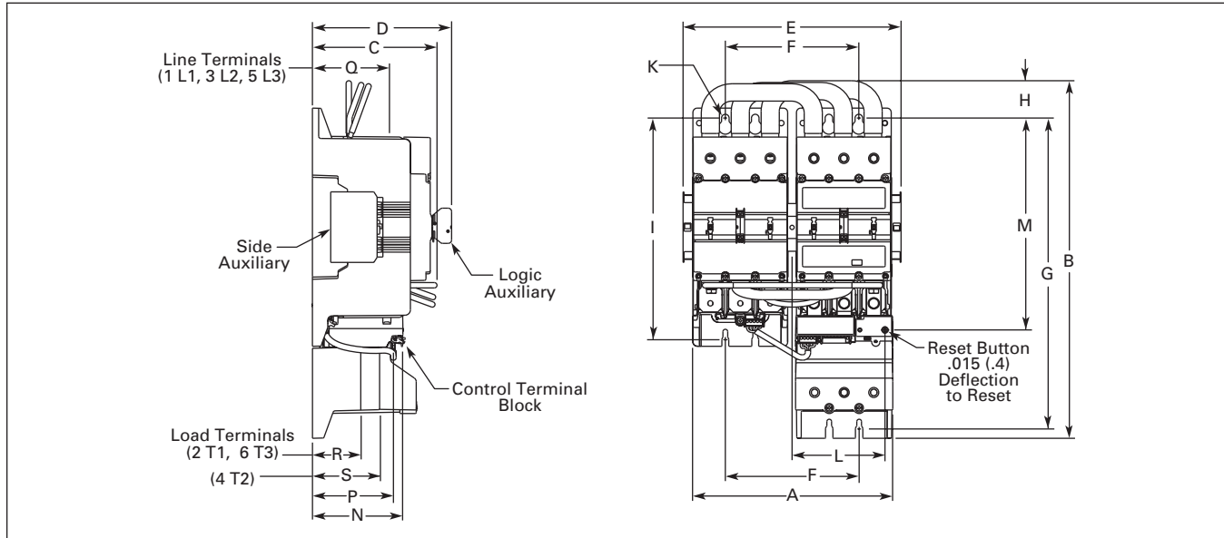
Figure 17. Approximate Dimensions in Inches (mm)
